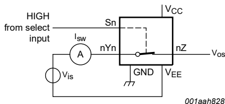
Fig. 12. Test circuit for measuring ON-state current
